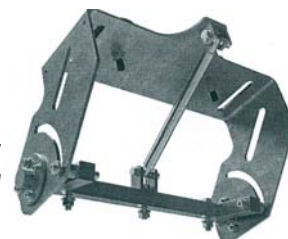
Crane Damper Bracket
